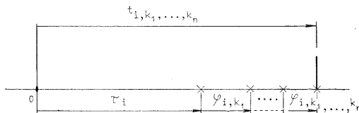
Fig. 4. Determination of pulse position with respect to the time axis origin. For figure to be easy to survey the variables \phi are chosen to be positive only. However, this need not always be the case because for some reference point positions the variables \phi can be both positive and negative.
